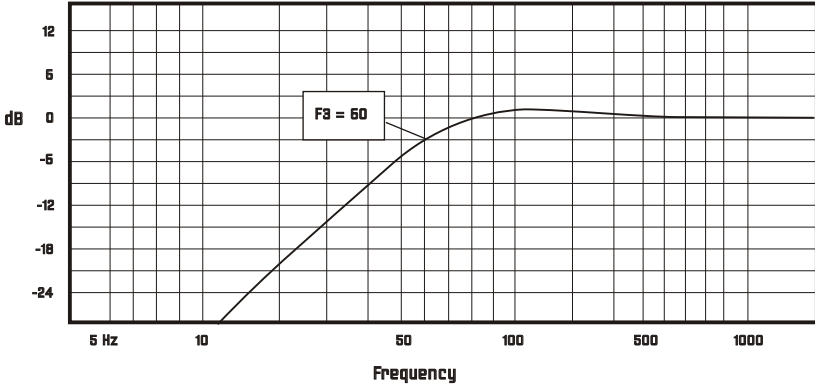
ELW1214P Amplitude Response (dB/Hz)
